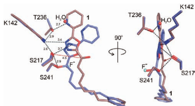
Figure 7. Cocrystal structure of covalently bound FAAH-1 (in blue) and noncovalently bound FAAH-1 (in light brown) display the differences in cytosolic port water H-bonds with the oxadiazole core.
