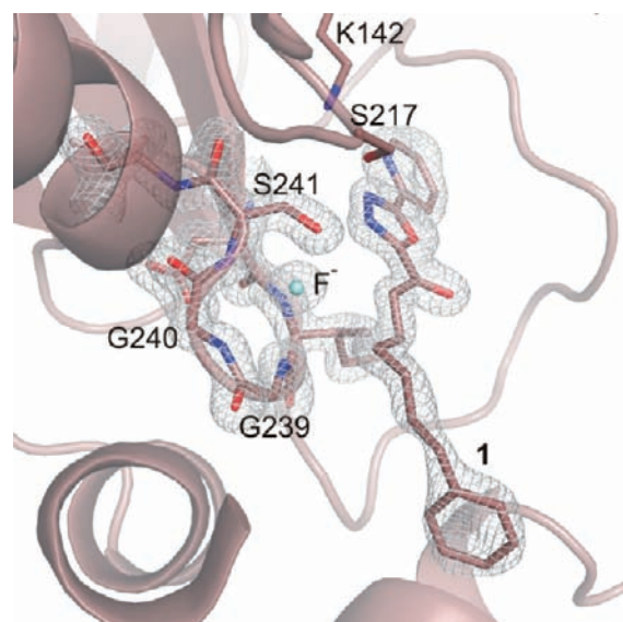
Figure 5. FAAH active site with noncovalently bound 1 and the proposed bound fluoride. The 2F_o - F_c electron density maps for noncovalently bound 1 at 1.5\sigma contour are shown with white meshes.
