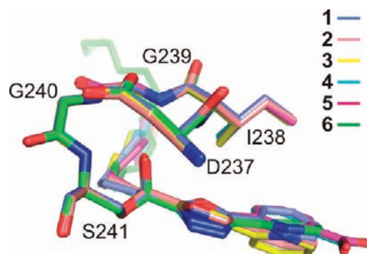
Figure 4. Superposition of the oxyanion holes for covalently bound 1 and the five prior structures of FAAH covalently bound to oxo(dia)zole inhibitors 2–6.
