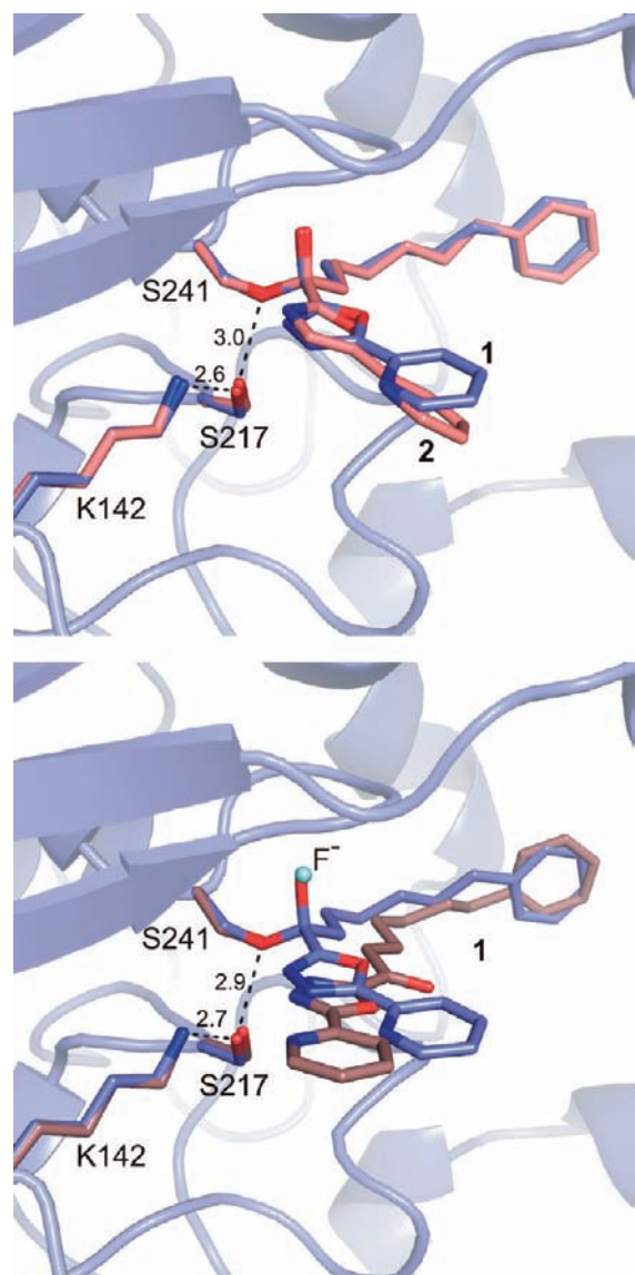
Figure 2. Top: Overlay of inhibitor 1 in the two bound states. Bottom: Overlay of covalently bound 1 and 2 (OL-135). Covalently bound inhibitor 1 is shown in light blue, noncovalently bound inhibitor 1 in brown, and 2 in pink. Interatomic distances of the noncovalent structure (top) and covalent structure (bottom) are shown with dashes and measured in Å.
